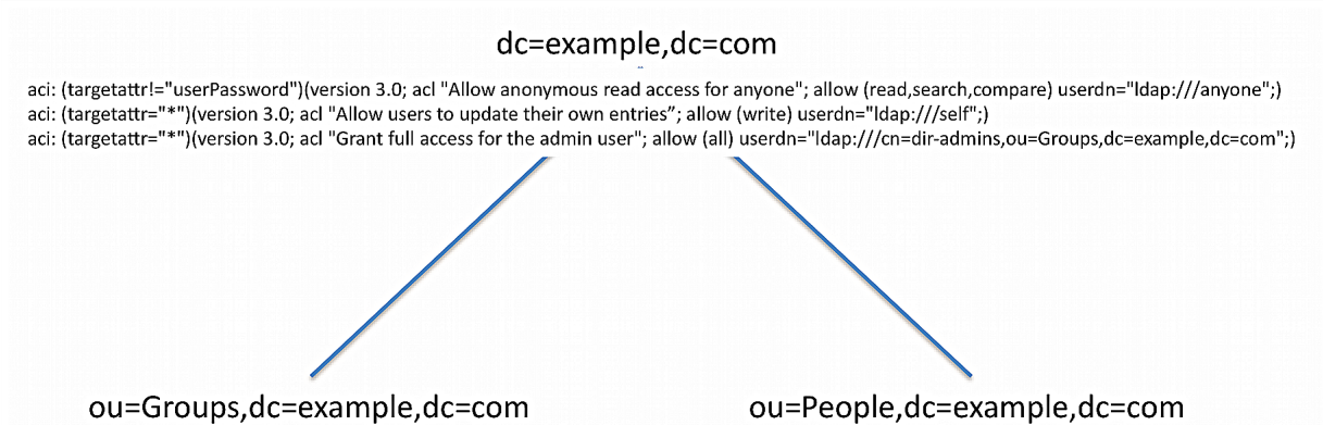
Figure 6: ACI
