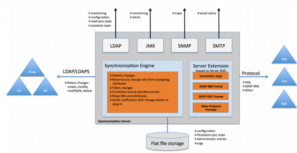
Notification Mode Architecture
